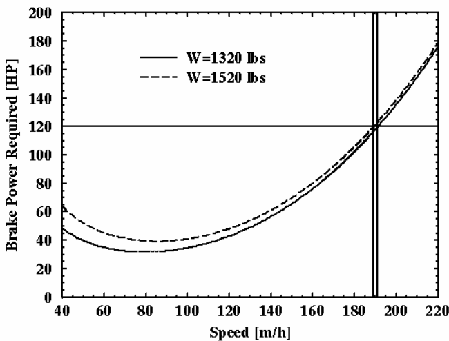
Figure 2: Plot of brake horsepower required versus speed for an RV-6 at weights of 1320 pounds and 1520 pounds
